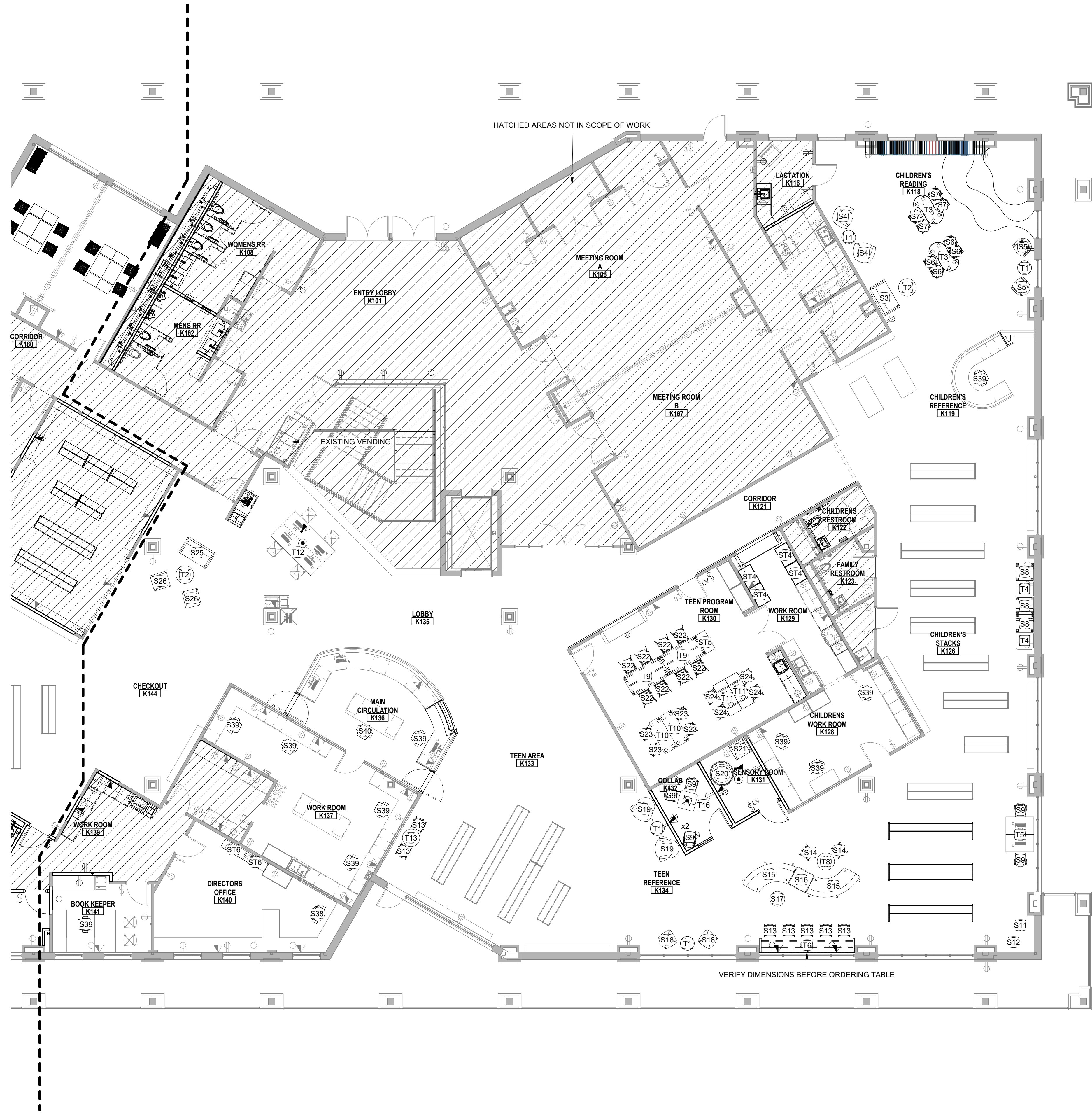
KPL - First Floor Furniture Plan - Unit A
